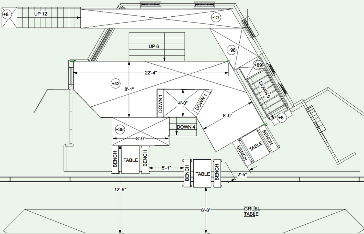
WORKHOUSE GROUNDPLAN
