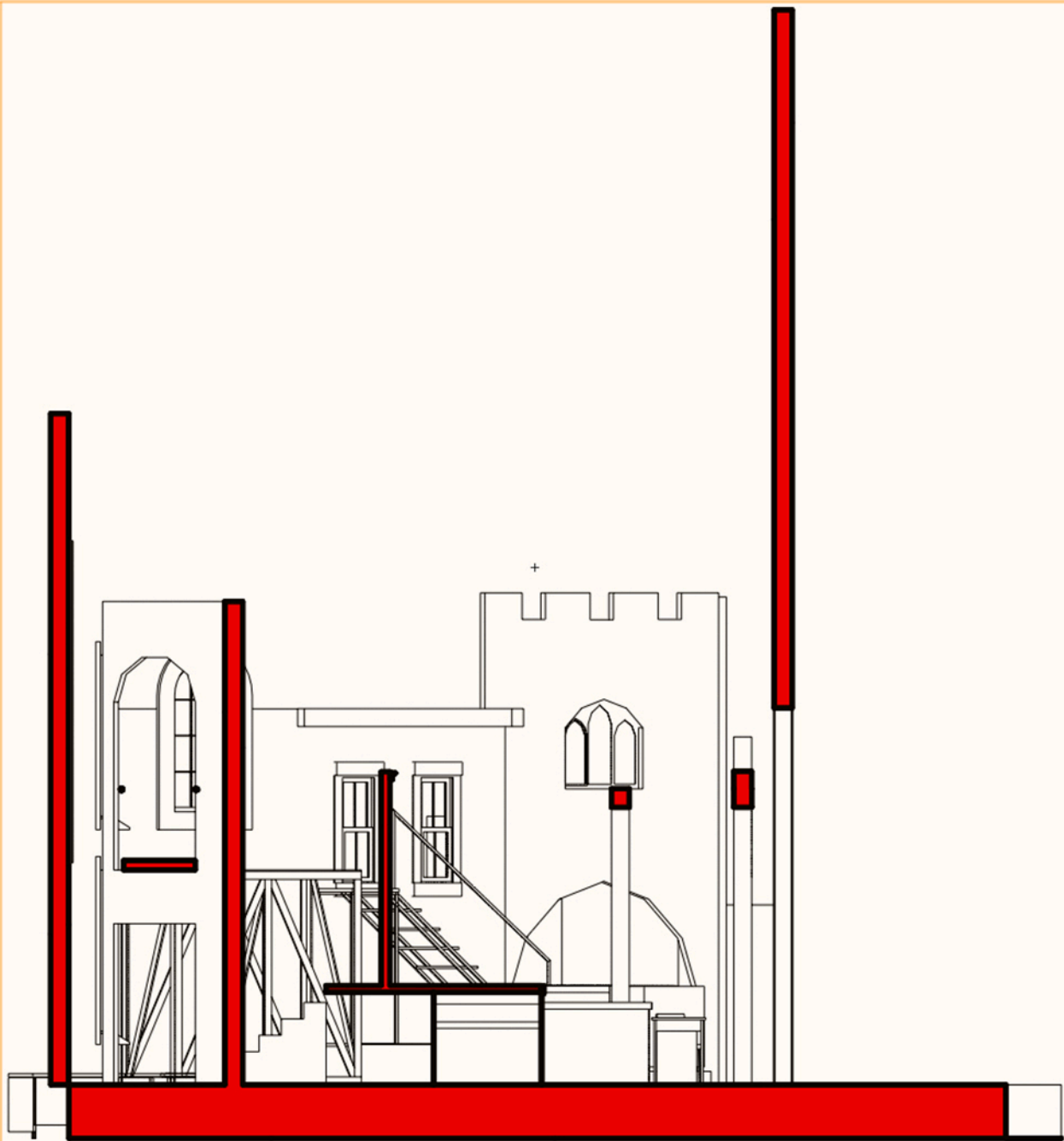
① South Section Thieve's Kitchen Scale: 1/4" = 1'-0"
