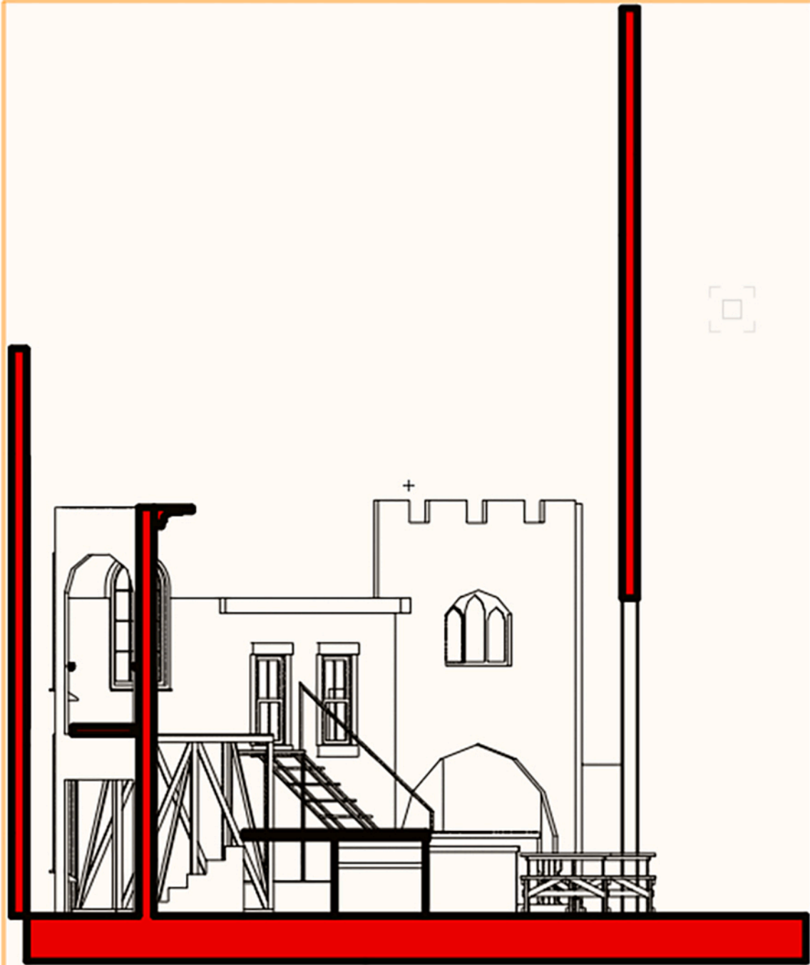
① South Section Scene 1 Scale: 1/4" = 1'-0"
