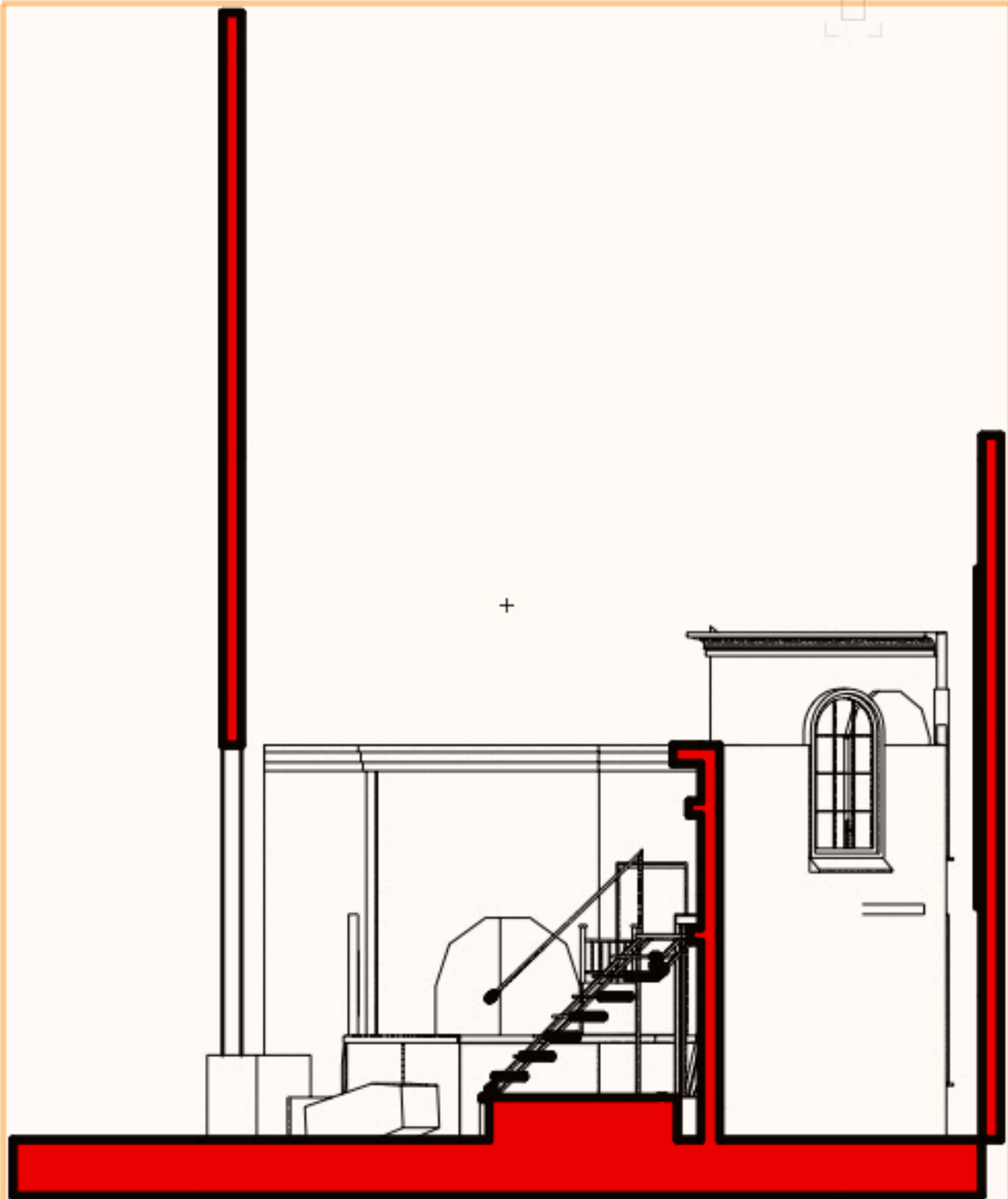
1 Sowerberry North Section Scale: 1/4" = 1'-0"
