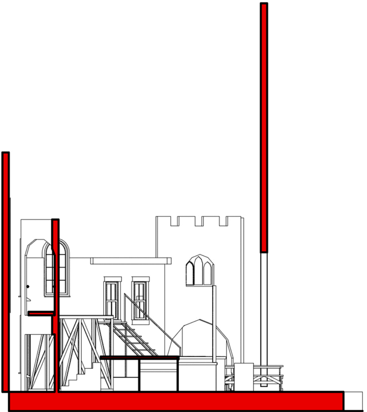
1 South Section Public House Scale: 1/4" = 1'-0"
